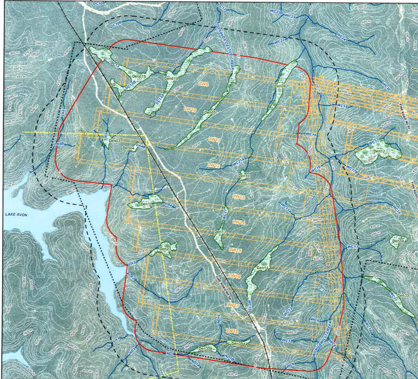
Figure 1: Site and Key Surface Features Plan
